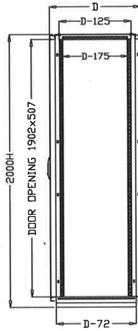
RIGHT VIEW
