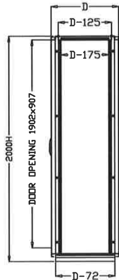
RIGHT VIEW
