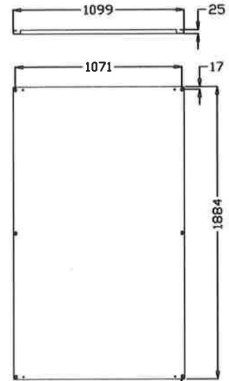
12x20 DBLONG FOR MOUNTING MOUNTING PLATE
