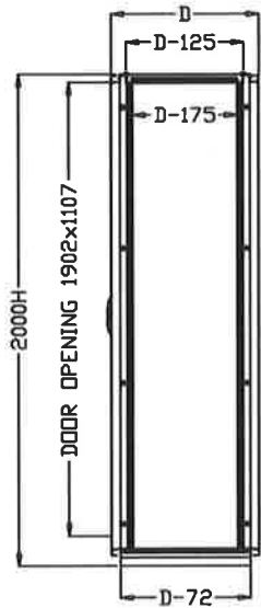
RIGHT VIEW
