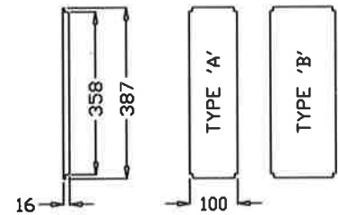
GLAND PLATE
