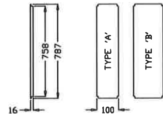
GLAND PLATE
