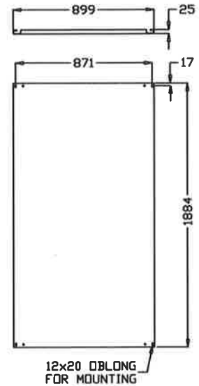
MOUNTING PLATE
