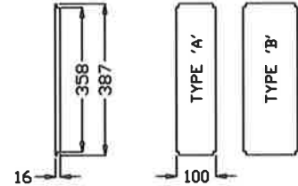
GLAND PLATE
